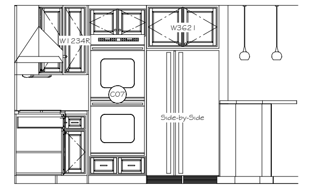
KITCHEN VIEW "C" @ 1/4" = 1' - 0"
