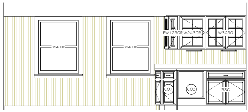
KITCHEN VIEW "A" @ 1/4" = 1' - 0"
