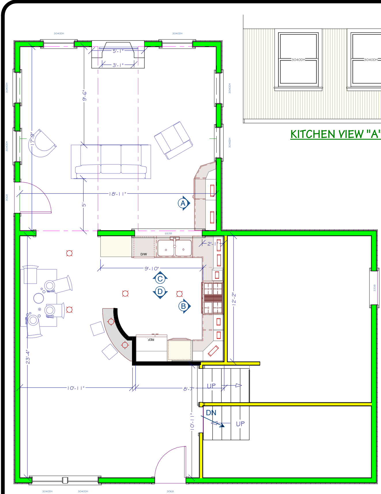
PROPOSED FLOOR PLAN @ 3/16" = 1' - 0"
