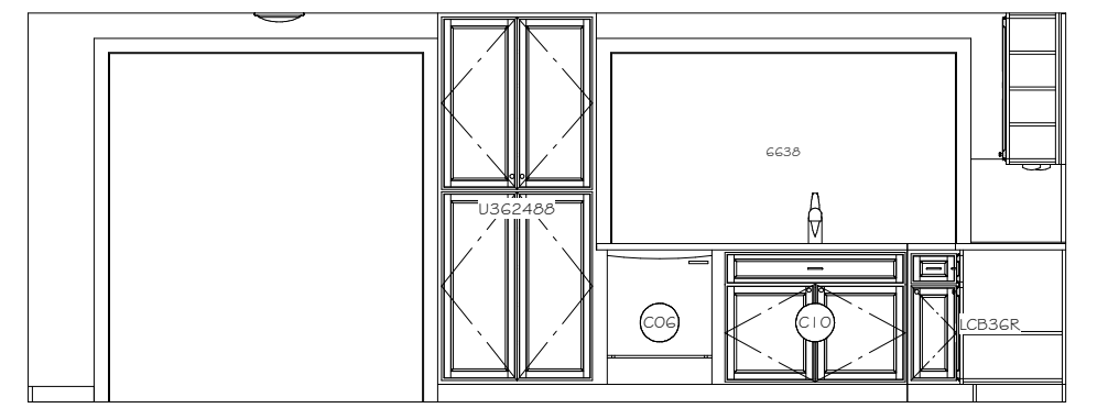
KITCHEN VIEW "D" @ 1/4" = 1' - 0"
