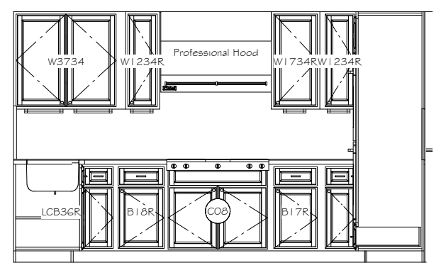
KITCHEN VIEW "B" @ 1/4" = 1' - 0"
